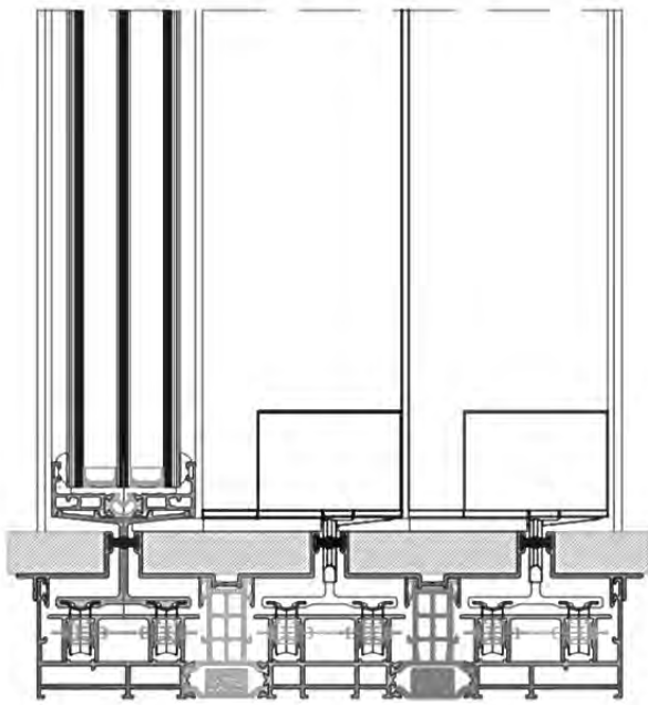
Door- cross-section KLAR VISION+
