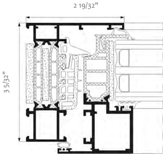
Window- cross-section KLAR C8o HO (HIDDEN SASH)
