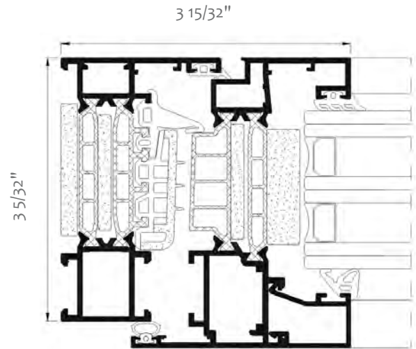
Window- cross-section KLAR C8o INDUSTRIAL
