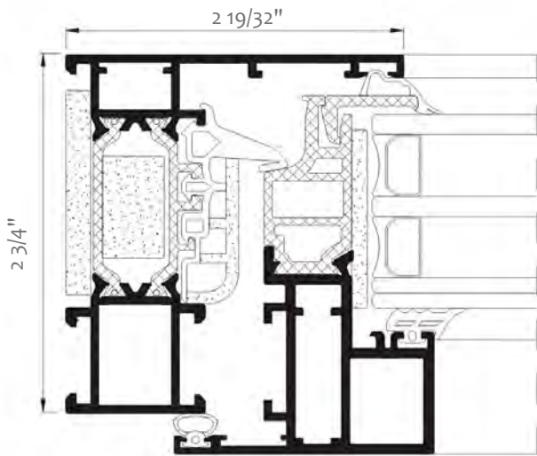
Window- cross-section KLAR C70 HO (HIDDEN SASH)
