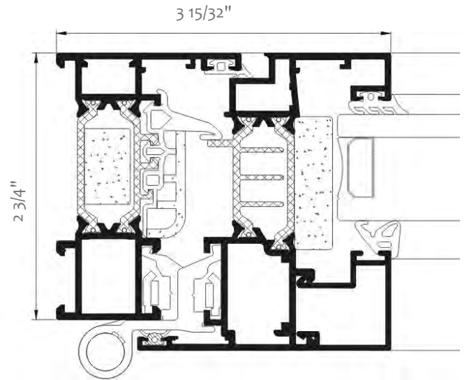
Window- cross-section KLAR C70 INDUSTRIAL
