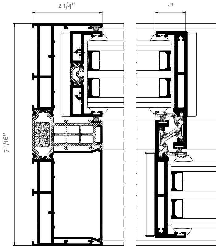
Door- cross-section KLAR VISION+
