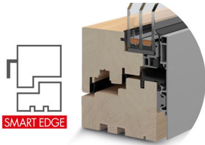
Timber-alu cross section of the SMART EDGE technology
