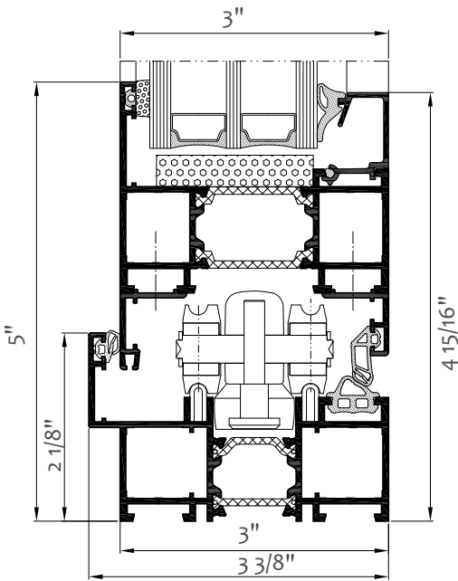
Door with edge sealing, bottom view-cross-section KLAR 86 FOLD LINE
