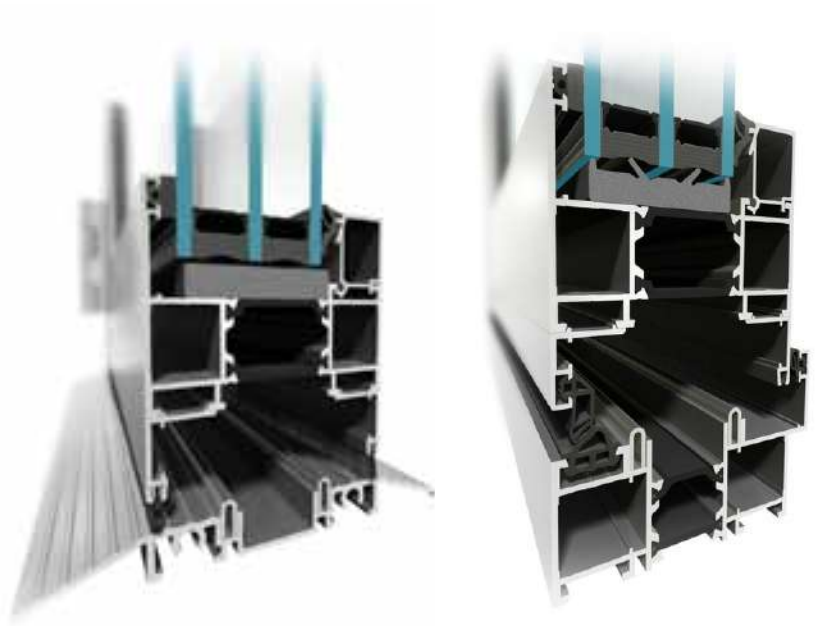
Door-KLAR 86 FOLD LINE U VALUE= from 0.26
