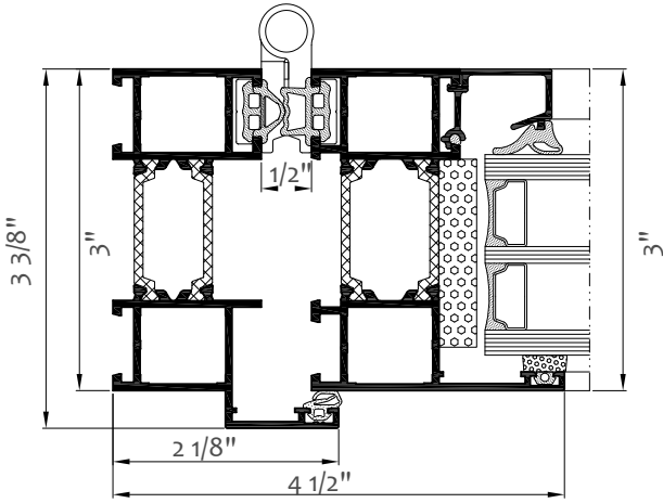
Door-SIDE VIEW - cross-section KLAR 86 FOLD LINE
