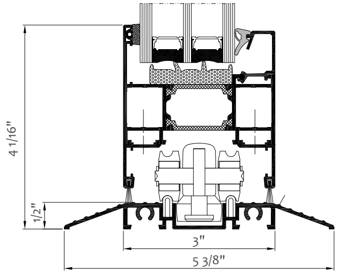
Door with low-level threshold, bottom view-cross-section KLAR 86 FOLD LINE
