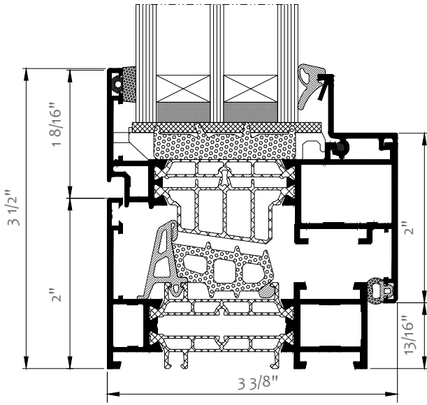
Window – cross-section KLAR-86ST
