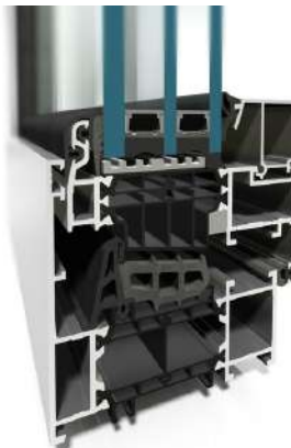
window KLAR'S-86US U value= 0.17
