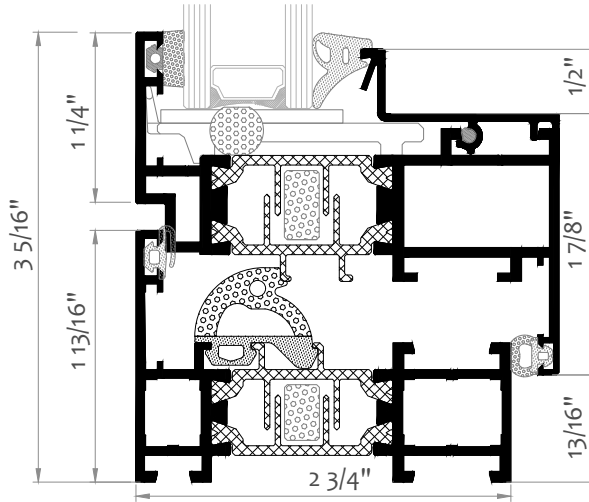
Window – cross-section KLAR-70 Hi
