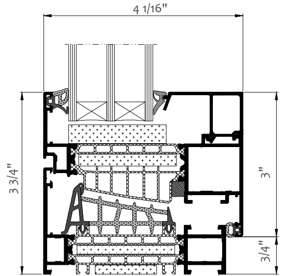
Window – cross-section KLAR-104 PASSIVE Aero
