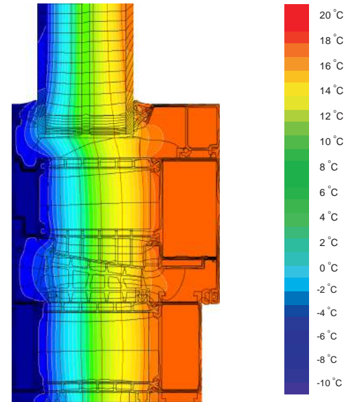
Isotherm distribution MB-104 Passive Aero
