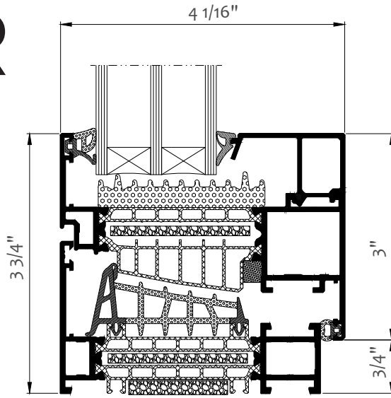
Window – cross-section KLAR-104 PASSIVE SI
